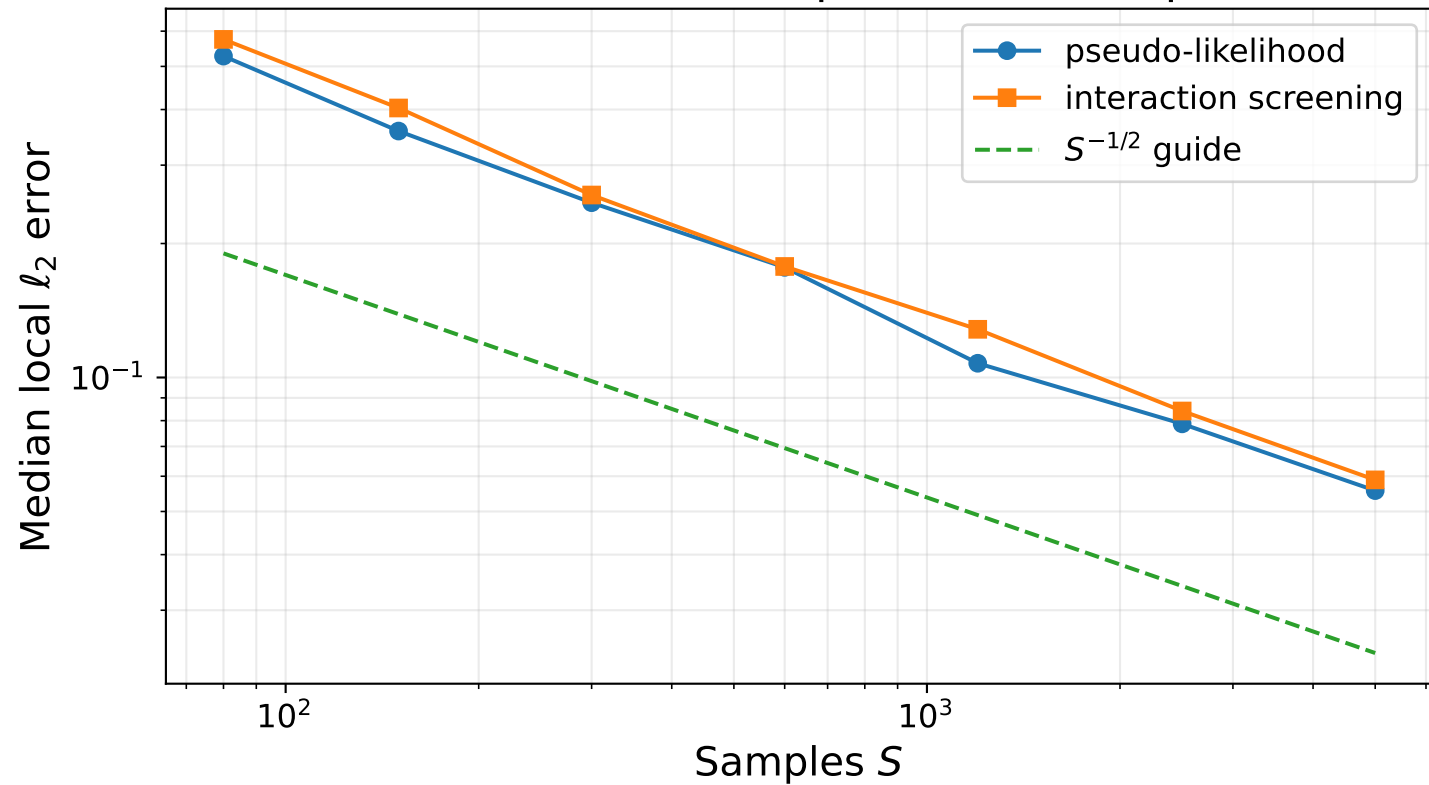
Both local estimators improve with sample size
