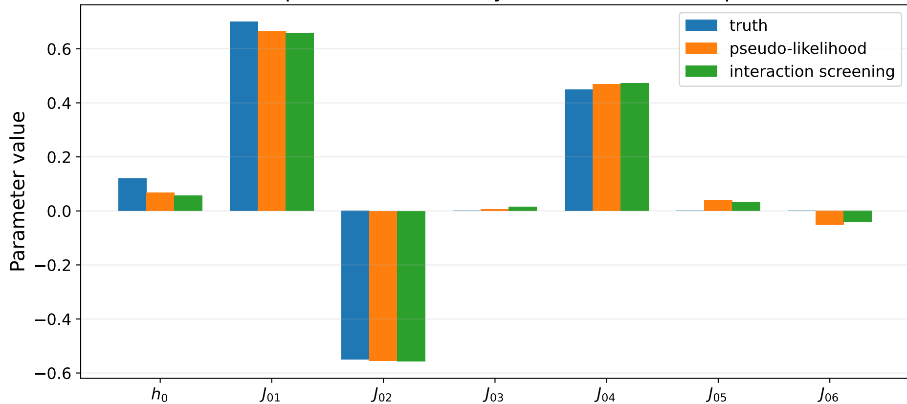
Local parameter recovery from S = 1200 samples
