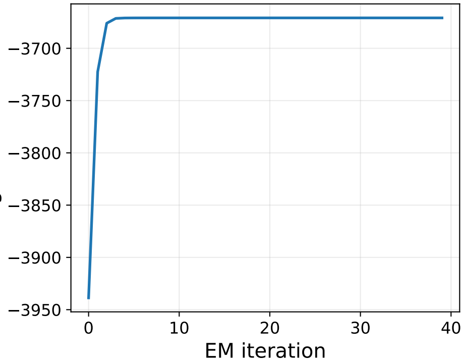
EM increases the observed-data likelihood
