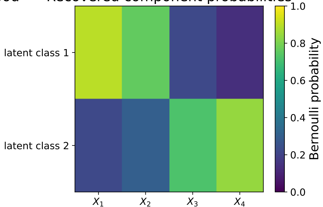
Recovered component probabilities
