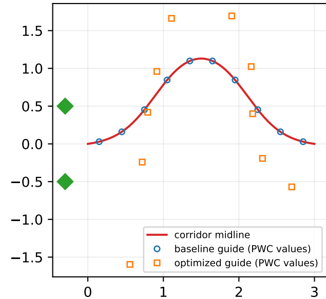
Guide geometry + entrance modes (◆)
