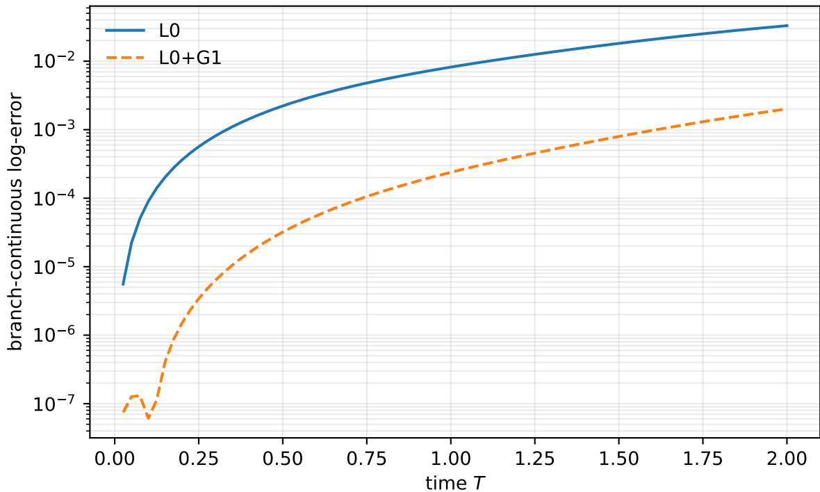
Driven anisotropic star, d = 6
