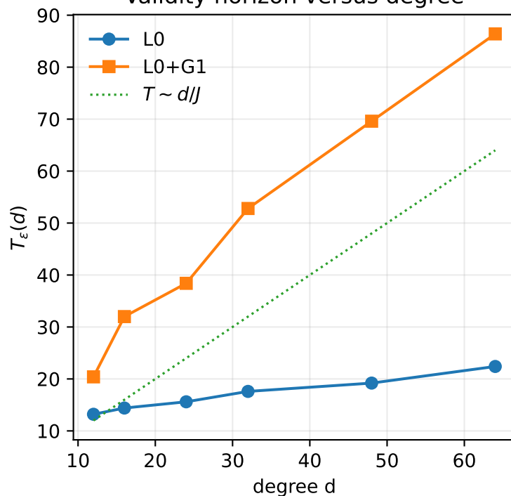
Validity horizon versus degree
