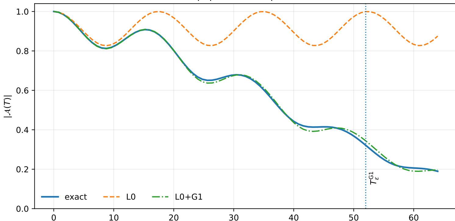
Error growth; threshold \epsilon = 0.10
