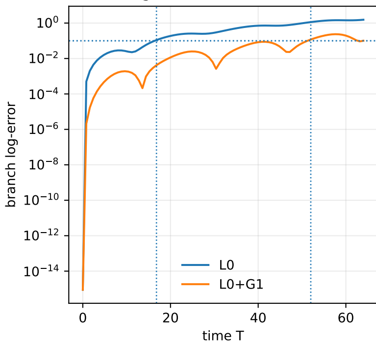
Error growth; threshold \epsilon = 0.10
