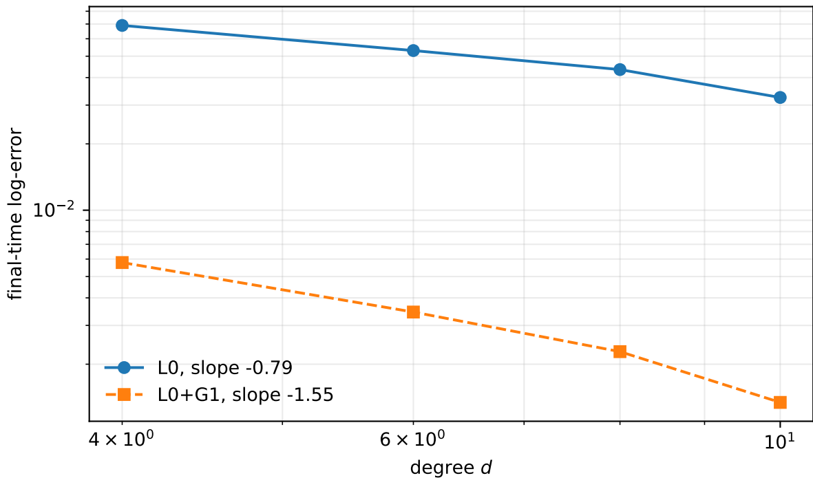
Driven-star final-time scaling, T = 2
