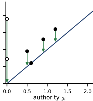
(c) deflation: delete noise lower bound, if curvature holds
