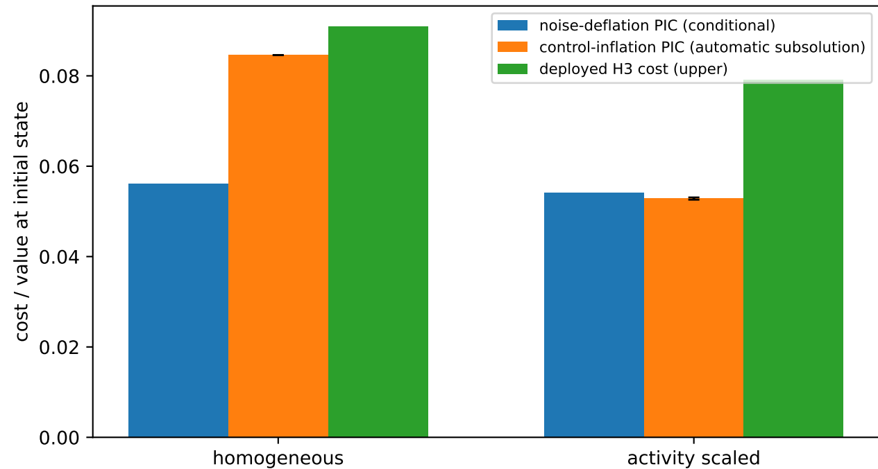
H3: dual PIC relaxations at nominal noise
