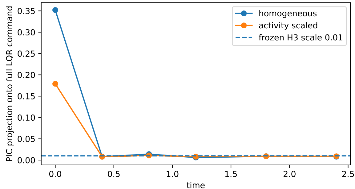
Sparse PIC feedback estimates
