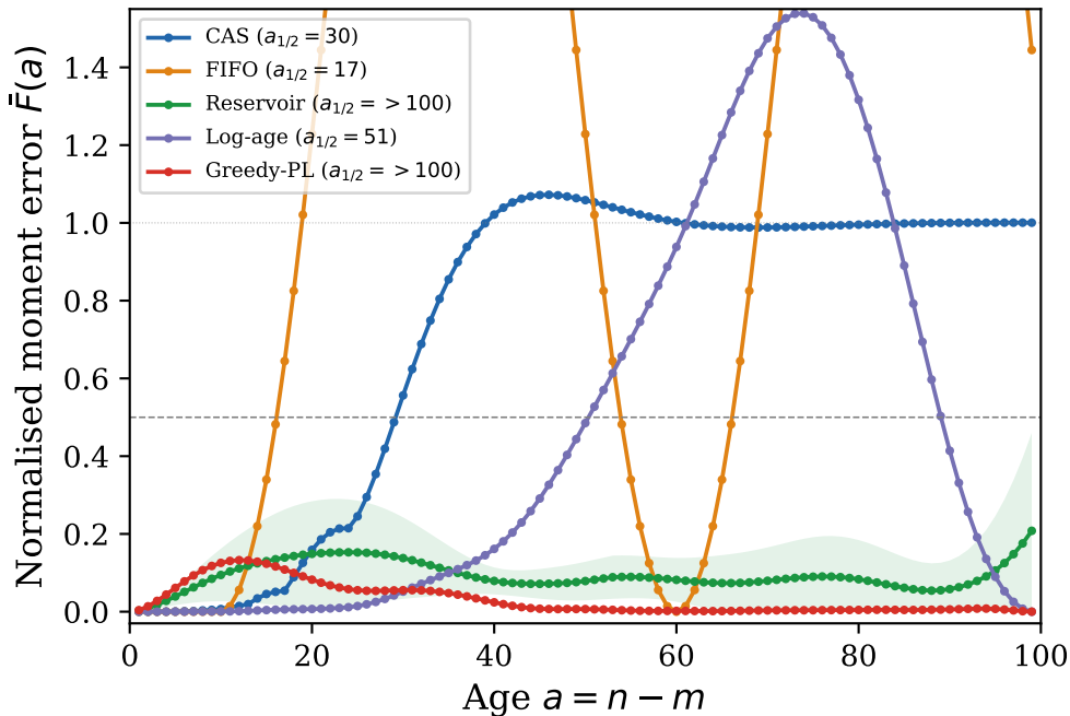
Memory-matched baselines: K = 1 , B = 11 GM states
