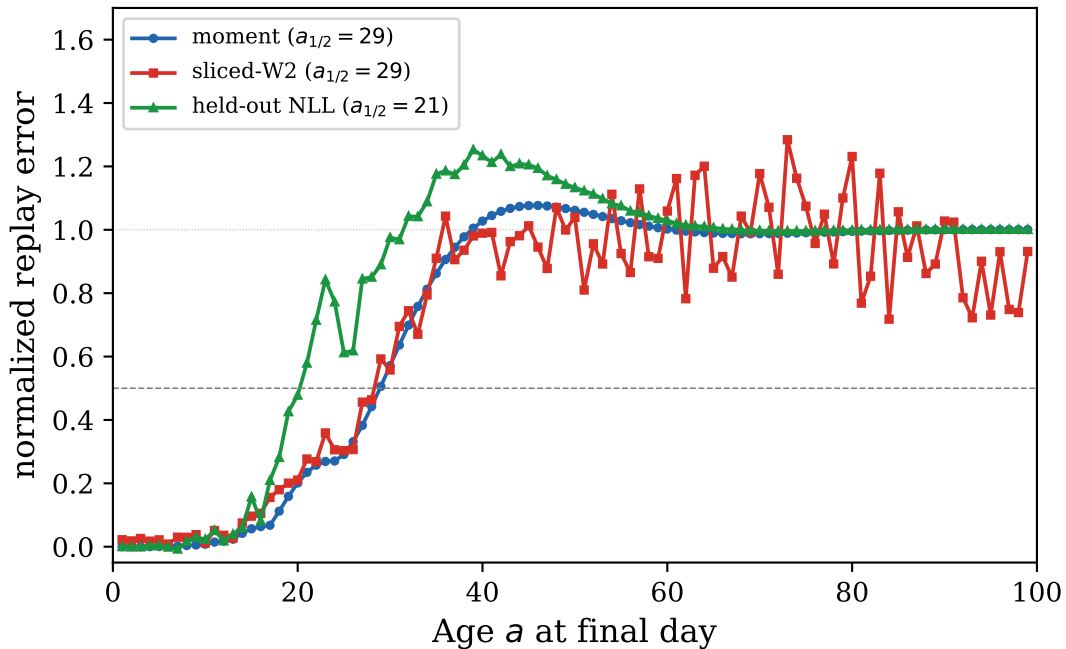
K=3 default: final-day metric comparison
