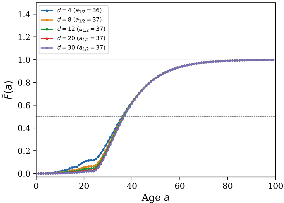
(a) MNIST age curves vs PCA dimension
