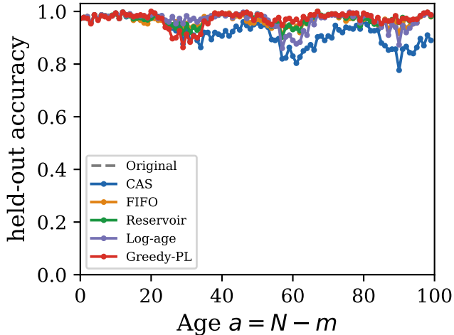
(a) Latent classification
