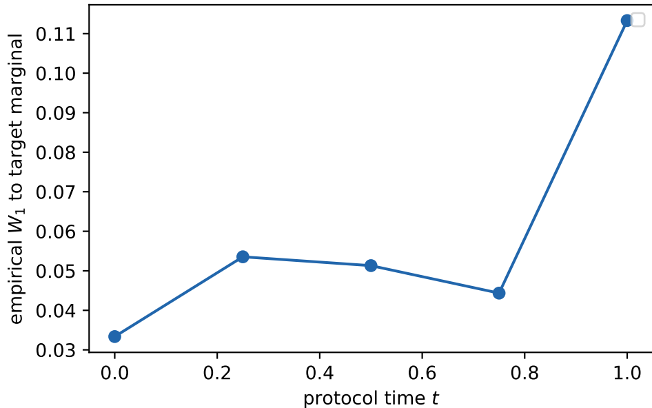
SDE marginal validation: time-varying weights
