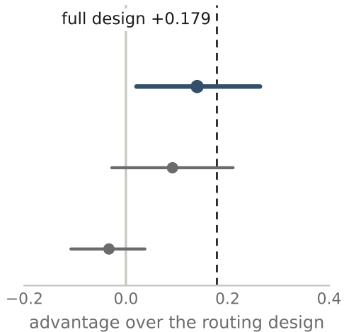
cloud (claude-sonnet-4-6)
