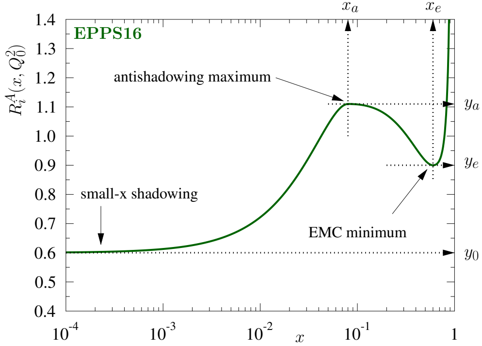
Figure 10: Illustration of the EPPS16 R_q^A(x, Q_0^2) fit function. Figure taken from Reference [17].
