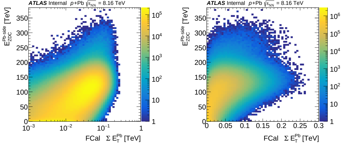
Figure 28: Correlation between the Pb going neutral forward energy ( E_{\text{ZDC}}^{\text{Pb-side}} ) and the transverse energy accumulated in the Pb-going FCal arm ( E_{\text{T}}^{\text{Pb}} ) for the p+\text{Pb} orientation. E_{\text{T}}^{\text{Pb}} is binned in logarithmic (left) and linear (right) fashion. E_{\text{ZDC}}^{\text{Pb-side}} is normalized to the single neutron peak in order to display energy in terms of number of neutrons.
