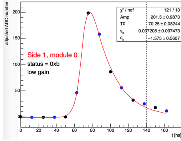
Figure 25: Example of a fitted ZDC pulse, taken from [ATL-COM-PHYS-2019-1454]
