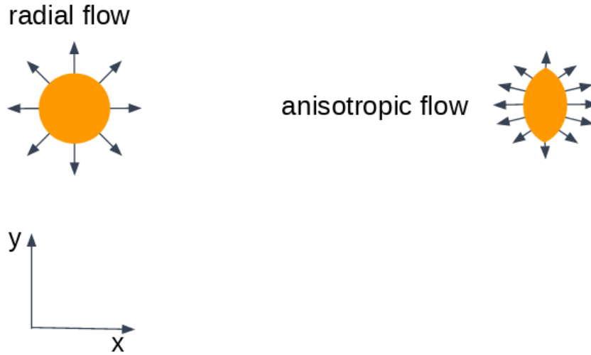
Figure 20: Schematic illustration of particle flow in a heavy-ion collision. Taken from Ref. [QGP:collisionTimeline].
