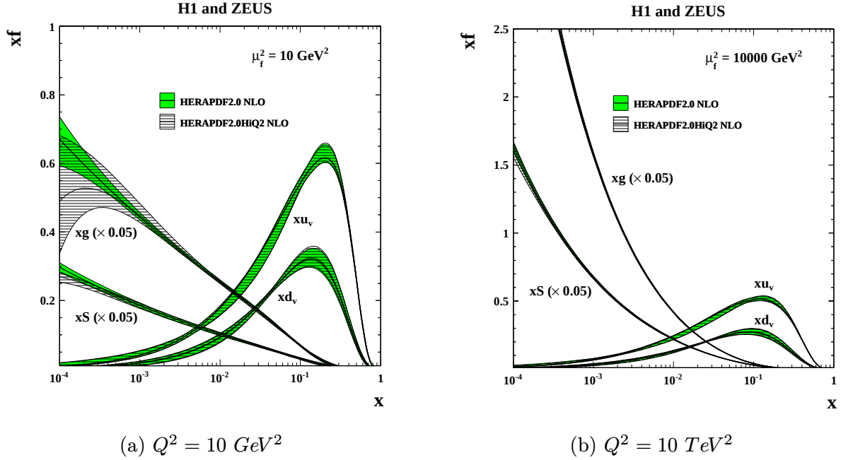
Figure 8: Proton PDFs at two factorization scales, showing the scale evolution predicted by the HERAPDF analysis. Figure from H1 and ZEUS Collaborations, arXiv:1506.06042v3 [ HERAF2 ].
