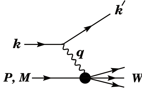
Figure 4: Schematic diagram of deep-inelastic e^- + p scattering, where the electron has initial four-momentum k and the proton has mass M and four-momentum P . Taken from Reference [pdg].
