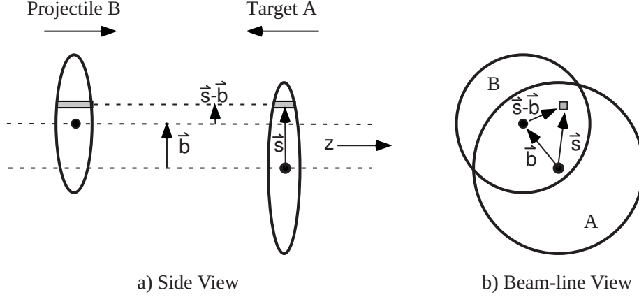
Figure 16: Schematic illustration of the ion collision geometry, reproduced from Ref. [Glauber].
