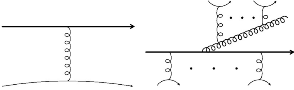
Figure 22: Schematic illustration of collisional (left) and radiative (right) energy loss of an energetic parton in the QGP. Taken from Ref. [QGP:JetQuenching].
