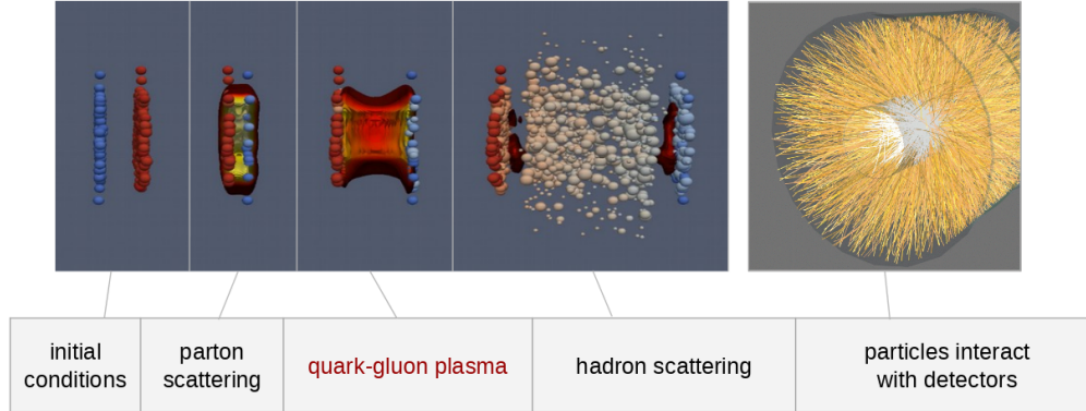
Figure 19: Cartoon illustrating the stages of a heavy-ion collision. Image from Reference [QGP:collisionTimeline] originally by H. Petersen and J. Bernhard, MADAI Collaboration.
