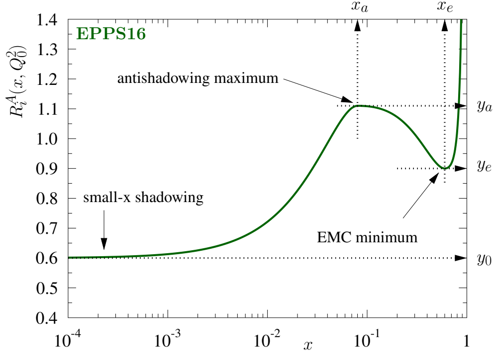
Figure 10: Illustration of the EPPS16 R_i^A(x, Q^2) fit function. Figure taken from Reference [nPDF].
