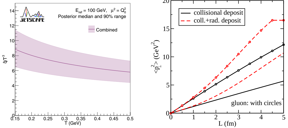
Figure 23: Left: Temperature dependence of \hat{q}/T^3 extracted through Bayesian analysis using jet and hadron measurements. Taken from Ref. [QGP:JetscapeQhat]. Right: Path-length dependence of the mean transverse momentum squared lost by quark and gluon jets through collisional energy loss alone and through collisional plus radiative energy loss. Taken from Ref. [QGP:Ldep].
