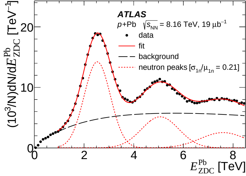
Figure 27: ZDC background estimation for run 313100, taken from [HION-2024-11].
