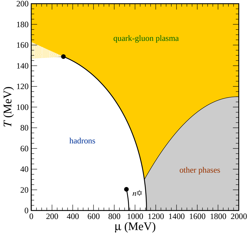
Figure 18: Phase diagram of nuclear matter in the baryon chemical potential ( \mu ) and temperature ( T ) plane. Taken from Ref. [QGP:Lattice2].
