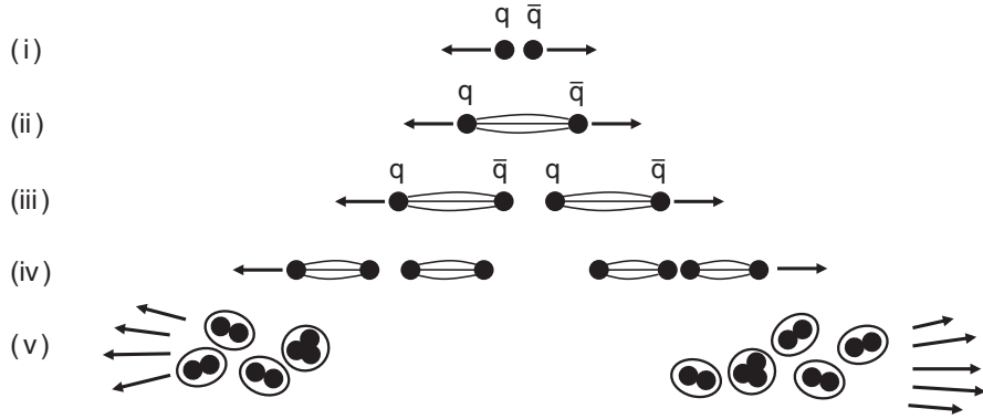
Figure 3: Schematic illustration of hadronization through the breaking of a color flux tube into quark–antiquark pairs and collimated streams of hadrons. Taken from Reference [thomsonqft].
