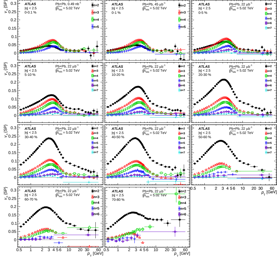
Figure 21: The v_n obtained as a function of transverse momentum p_T in 11 centrality intervals, from the most central at the top left panel to the most peripheral at the bottom right panel. Taken from Ref. [HION-2016-06].
