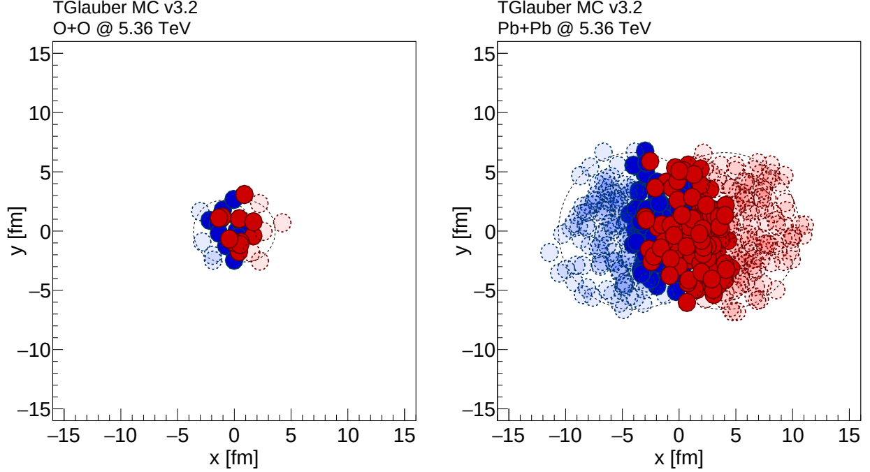
Figure 17: Distributions of nucleons generated with Glauber Monte Carlo in the x - y transverse plane. The two nuclei are shown in different colors, with the participants shown as darker circles. Results for O+O collisions (left) and Pb+Pb collisions (right) are shown. Figures provided by R. Longo.
