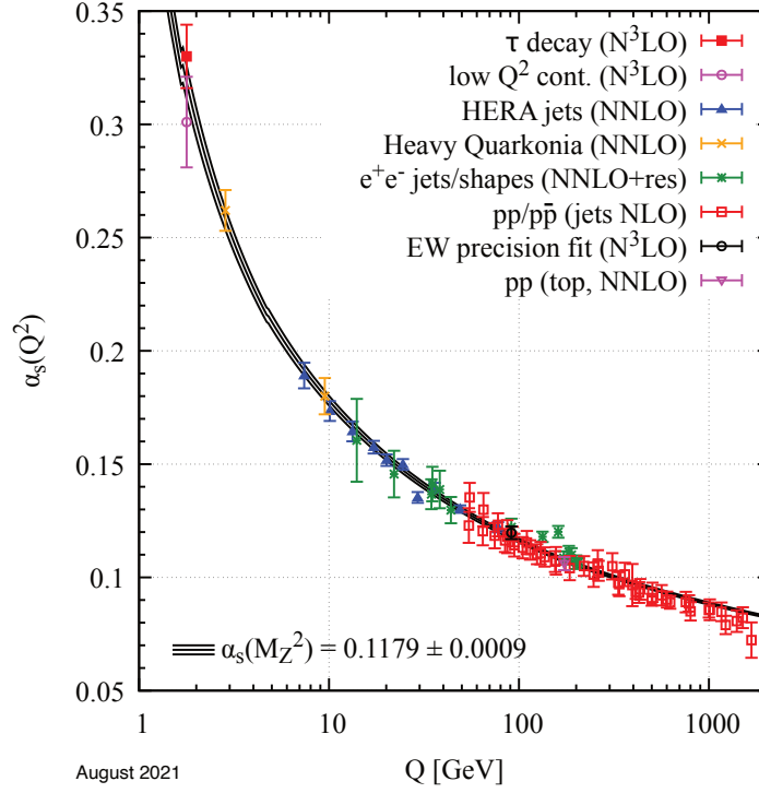
Figure 1: The running of the strong coupling \alpha_s as a function of the momentum-transfer scale, illustrating asymptotic freedom. Taken from Reference [pdg]
