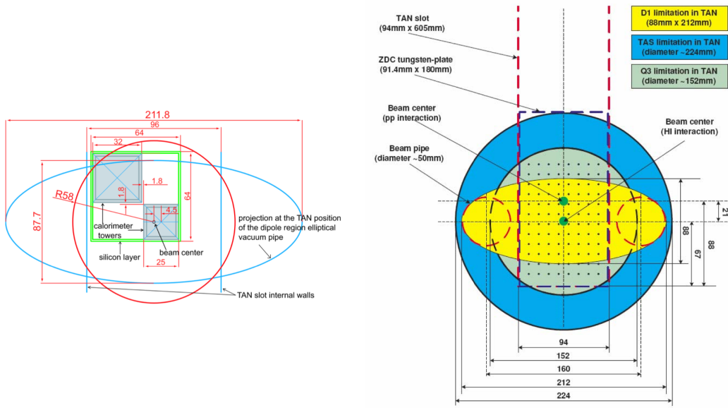
Figure 19: Detector geometry for LHCf Arm2 [Cekmecelioglu:2867369] (left) and the ATLAS ZDC [Jenni:1009649] (right), viewed from the ATLAS interaction point. Distances are given in mm. The blue oval in the left image corresponds to the boundary of the yellow oval in the right image. The active area of LHCf is represented by the filled blue squares, and the active area of the ZDC is bounded by the purple dashed line.
