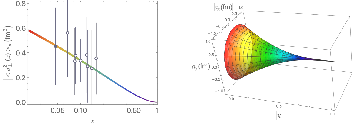
(a) Model prediction compared with CLAS and HERMES data.
