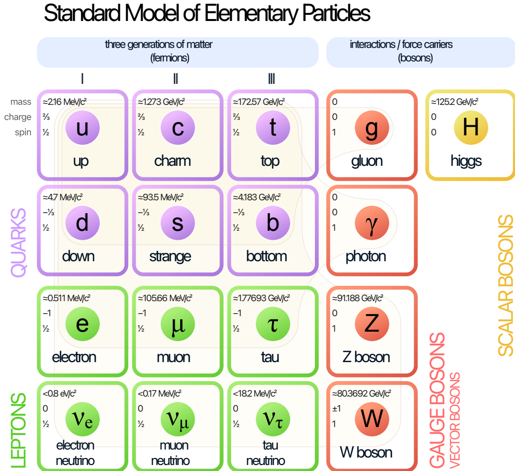
Figure 1: The elementary particles and force carriers of the Standard Model. Adapted from Ref. [1].
