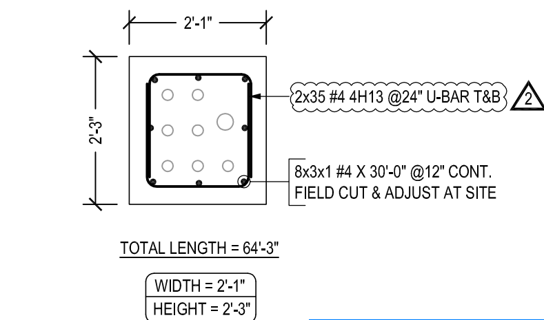
TYPICAL DUCT BANK DETAILS - 06C, 06E & 06G SCALE - 1/2"=1'-0" REF:00-T-07-705 & 00-E-03-301 TO 308
