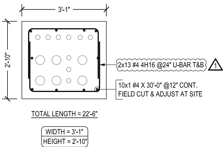
TYPICAL DUCT BANK DETAILS - 25A SCALE - 1/2"=1'-0" REF:00-T-07-705 & 00-E-03-301 TO 308
