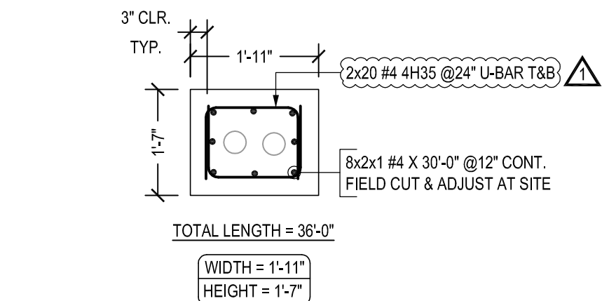
TYPICAL DUCT BANK DETAILS - 21L SCALE - 1/2"=1'-0" REF:00-T-07-705 & 00-E-03-301 TO 308
