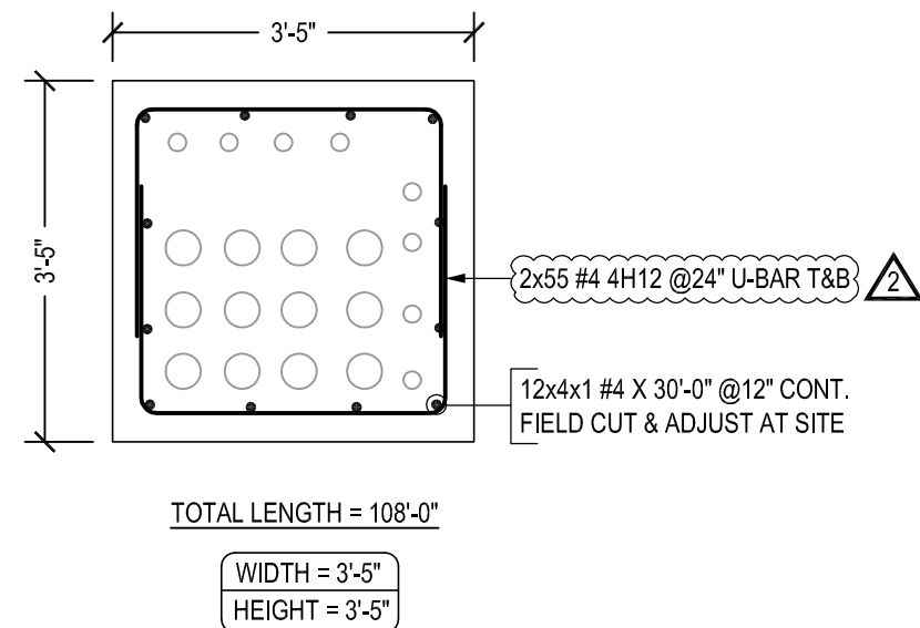
TYPICAL DUCT BANK DETAILS - 12A SCALE - 1/2"=1'-0" REF:00-T-07-705 & 00-E-03-301 TO 308
