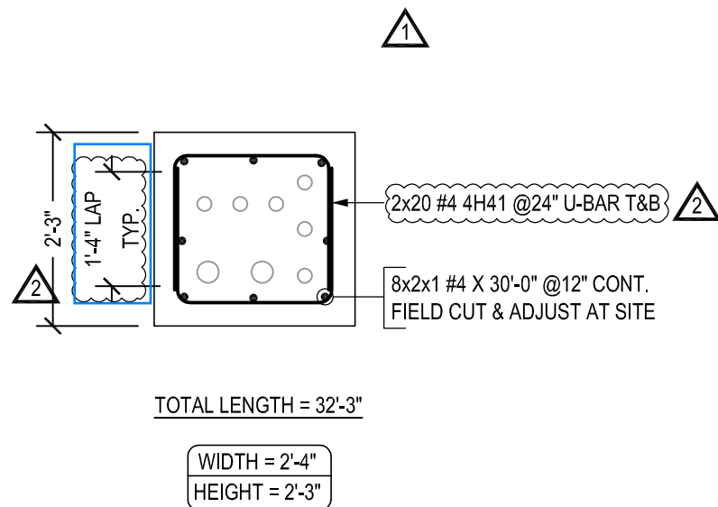
TYPICAL DUCT BANK DETAILS - 13B SCALE - 1/2"=1'-0" REF:00-T-07-705 & 00-E-03-301 TO 308
