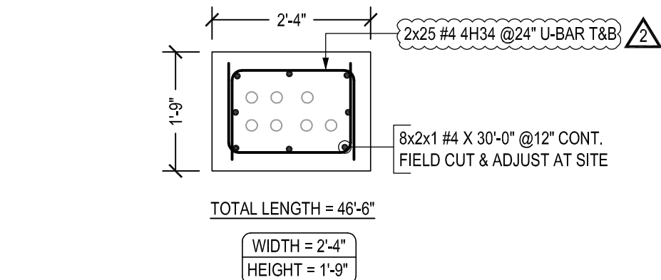
TYPICAL DUCT BANK DETAILS - 11C & 14B SCALE - 1/2"=1'-0" REF:00-T-07-705 & 00-E-03-301 TO 308
