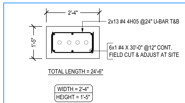
TYPICAL DUCT BANK DETAILS - 05B SCALE - 1/2"=1'-0" REF:00-T-07-705 & 00-E-03-301 TO 308
