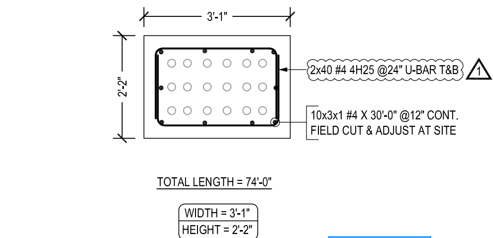
TYPICAL DUCT BANK DETAILS - 14A & 21A SCALE - 1/2"=1'-0" REF:00-T-07-705 & 00-E-03-301 TO 308
