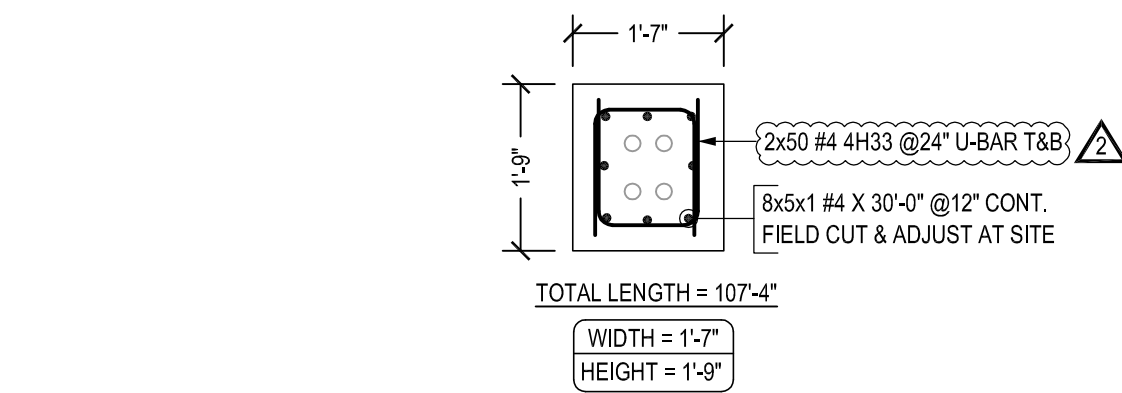
TYPICAL DUCT BANK DETAILS - 23A, 21F, 13A, 11D, 11G, 11H & 11I SCALE - 1/2"=1'-0" REF:00-T-07-705 & 00-E-03-301 TO 308
