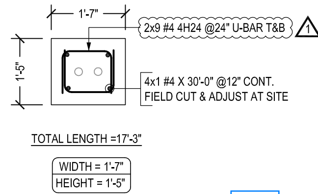
TYPICAL DUCT BANK DETAILS - 13C SCALE - 1/2"=1'-0" REF:00-T-07-705 & 00-E-03-301 TO 308
