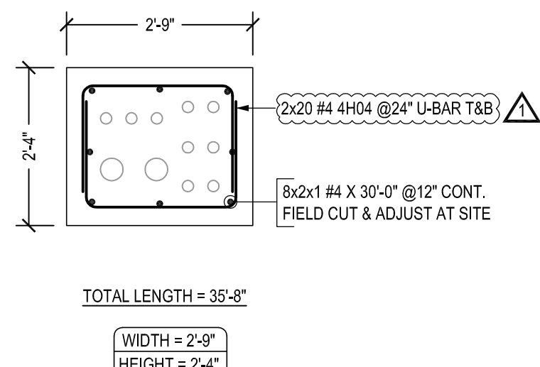
TYPICAL DUCT BANK DETAILS - 09A SCALE - 1/2"=1'-0" REF:00-T-07-705 & 00-E-03-301 TO 308
