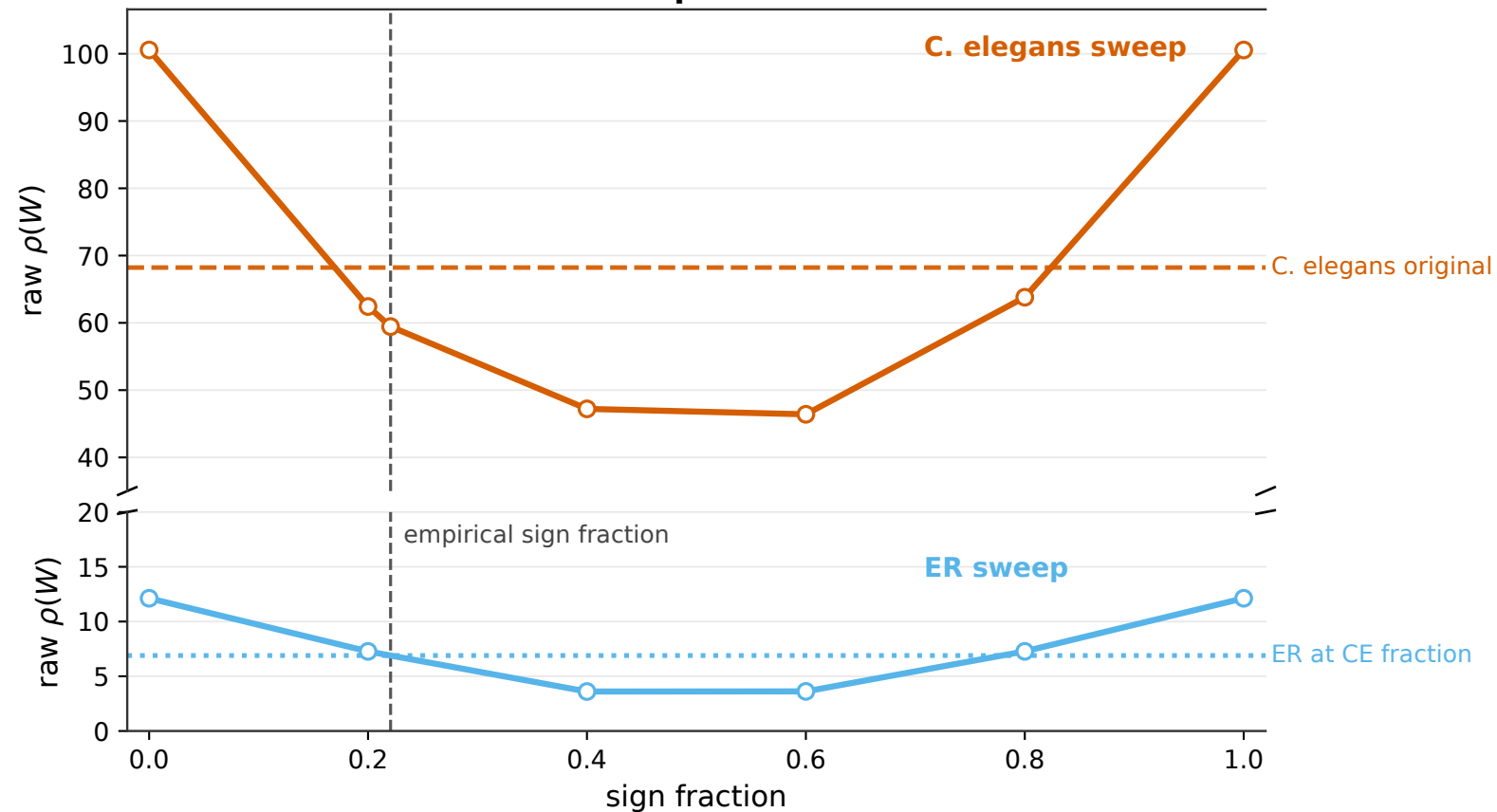
Mean raw spectral radius
