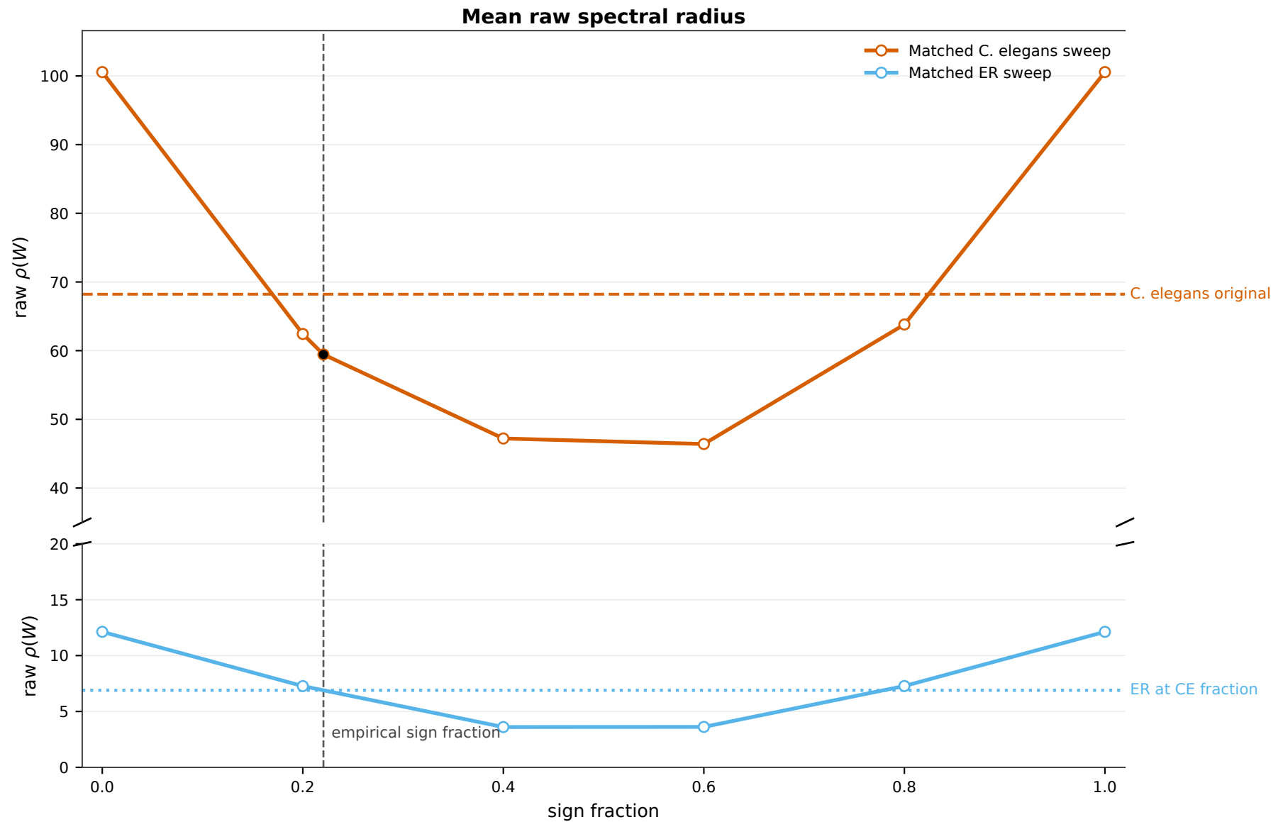
Sign-sweep quick look: the C. elegans sweep can cross below the original raw spectral radius before the empirical sign fraction
