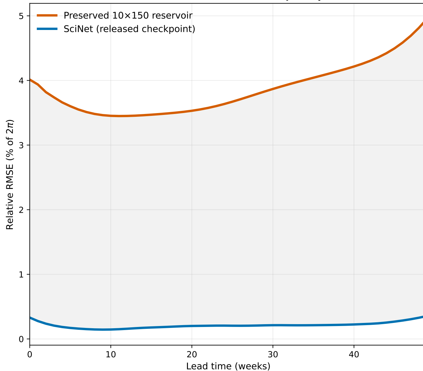
Error across the 50-week trajectory
