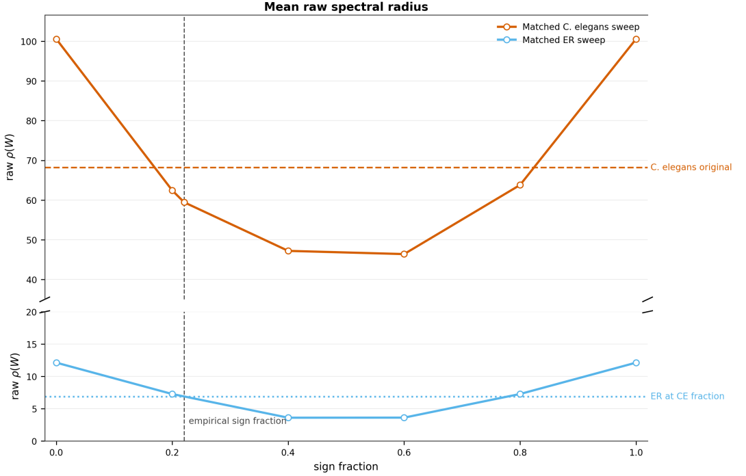
Figure 8: Quick look at the sign-sweep comparison between the C. elegans and C. elegans -matched ER topologies. The vertical dashed line marks the empirical negative-edge fraction. In the C. elegans sweep, the raw spectral radius can dip below the original baseline slightly before that fraction is reached because sign placement is simultaneously being randomized. The ER-matched sweep shows a smaller offset, consistent with signs already being effectively random relative to topology.
