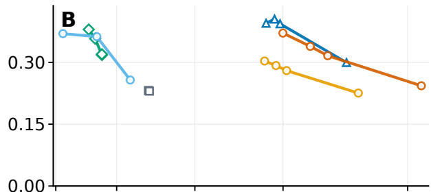
Mean CV
