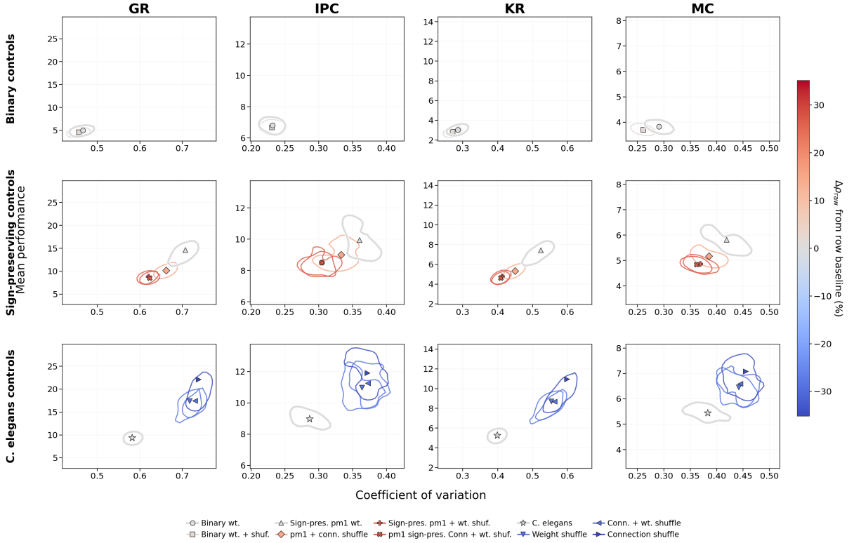
Figure 8: Performance–CV islands for the shuffle controls, shown with 50% density contours. Columns correspond to GR, IPC, KR, and MC. Rows show all-positive binary controls, sign-preserving signed-unit controls, and real-valued C. elegans controls. Contour color shows the percent change in raw spectral radius relative to the row baseline, \Delta\rho_{\text{raw}} ; blue indicates lower raw spectral radius and red indicates higher raw spectral radius.
