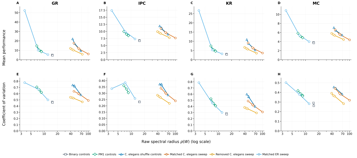
Figure 9: Relationship between raw spectral radius and reservoir behavior across sign-sweep and shuffle-control families. The top row shows mean task-agnostic performance as a function of raw spectral radius before normalization, \rho_{\text{raw}} , on a log scale. The bottom row shows the corresponding hyperparameter CV. Columns correspond to GR, IPC, KR, and MC. Lines connect points within experimental families and are not global fitted curves. Across families, lower \rho_{\text{raw}} generally coincides with higher performance and higher CV, while higher \rho_{\text{raw}} coincides with lower performance and lower CV.
