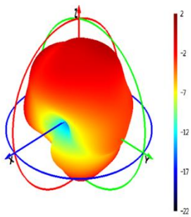
900 MHz
