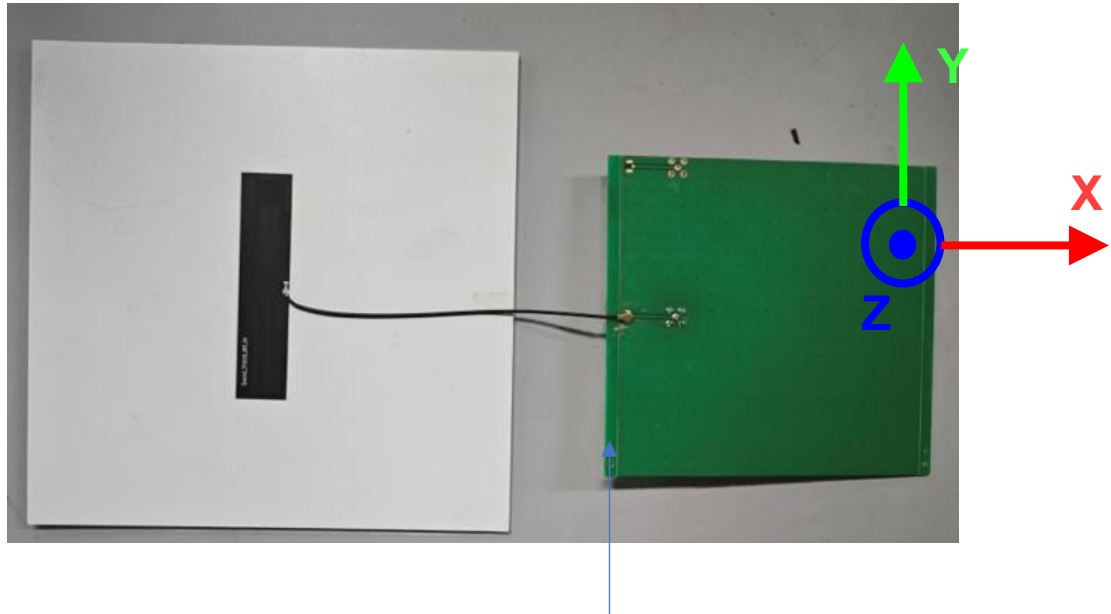
130 × 130 mm EVB
