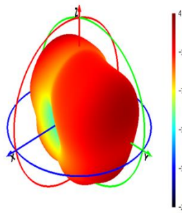
1740 MHz
