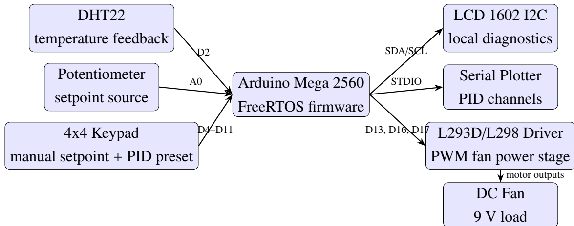
Figure 2.1 – System structural diagram for PID temperature regulation
