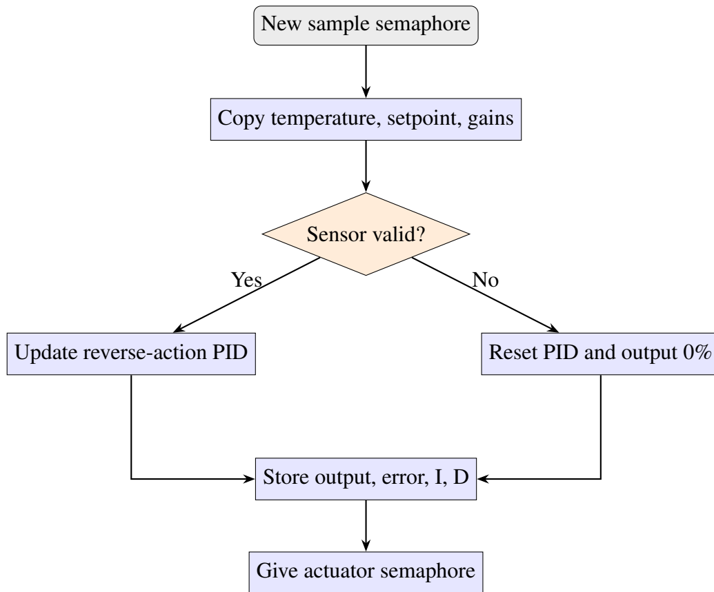
Figure 2.3 – Flowchart of the PID control task
