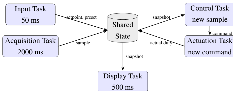
Figure 2.4 – FreeRTOS task data flow
