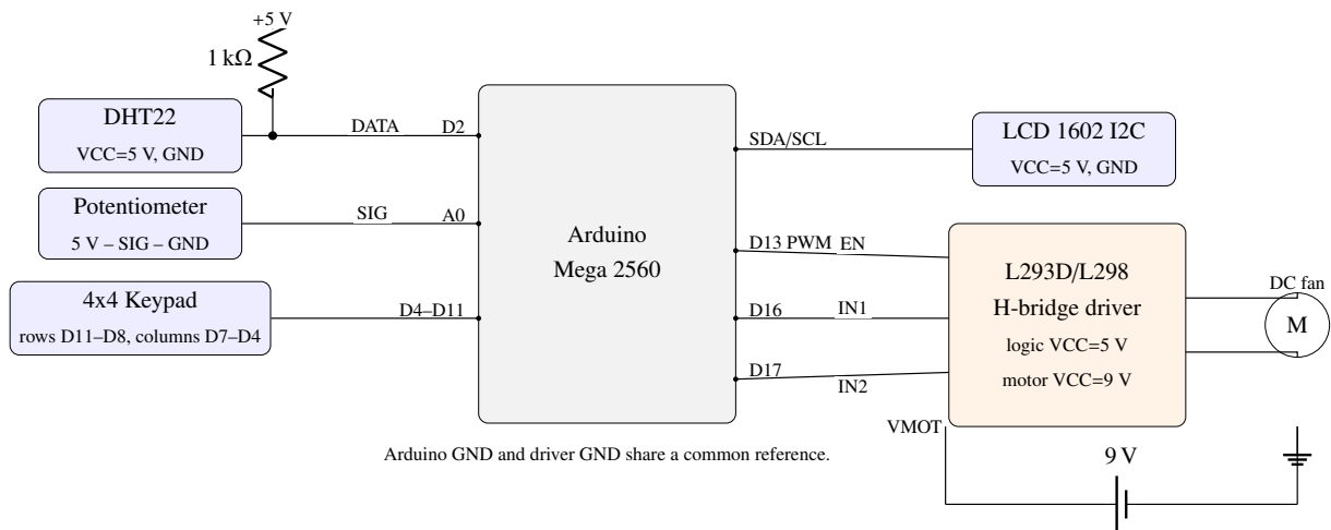
Figure 2.6 – Electrical schematic of the PID temperature control circuit
