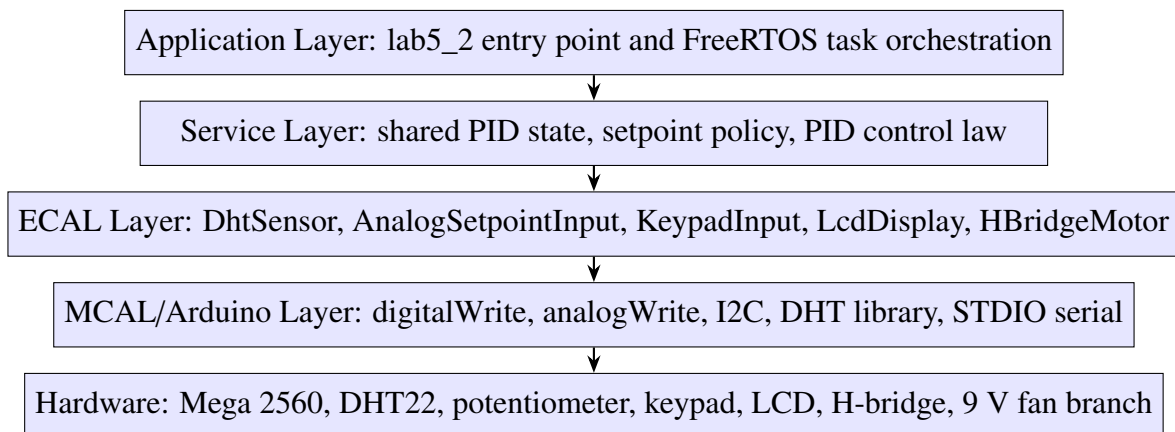
Figure 2.2 – Layered architecture of the PID control application
