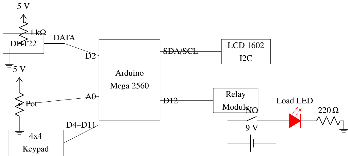
Figure 2.6 – Electrical schematic of the temperature control circuit
