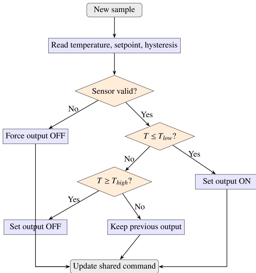
Figure 2.4 – Flowchart of the ON-OFF control algorithm with hysteresis
