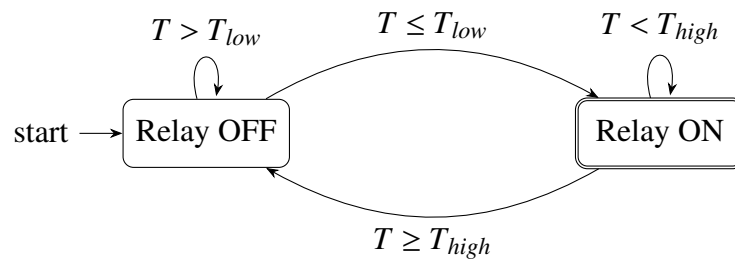
Figure 2.5 – Hysteresis controller state diagram
