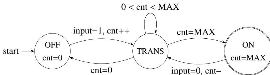
Figure 2.7 – Binary conditioner (debounce) state diagram
