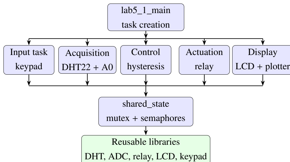
Figure 2.9 – Module responsibility map for the Lab 5.1 implementation
