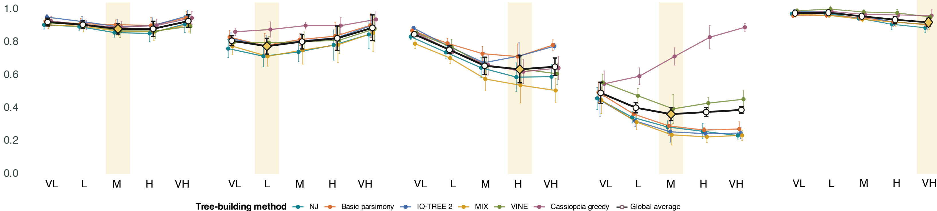
Mean normalized RF distance
