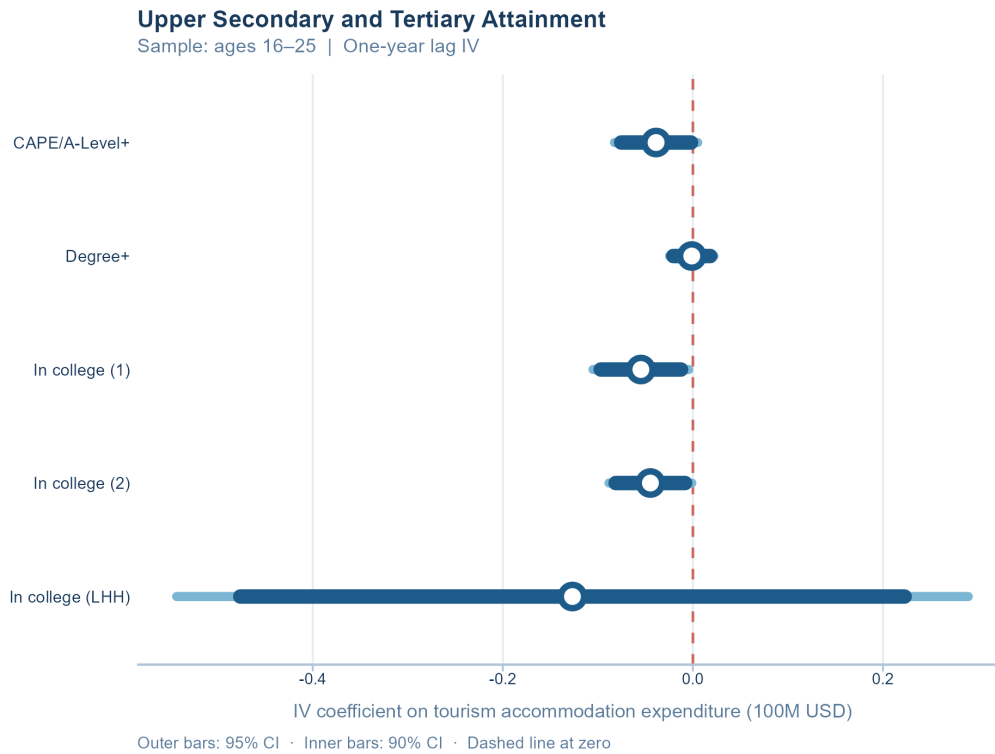
Figure 5: Upper Secondary and Tertiary Attainment: IV Coefficient Estimates Tourism expenditure coefficients (one-year lag) from the IV regressions. Wide bars show 95% confidence intervals; narrow bars show 90% intervals. Dashed line marks zero.
