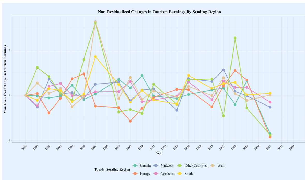
Figure 8: Graphs of Original Shift-Share Shocks
