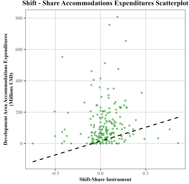
Figure 6: Scatterplot of the Shift-Share IV and Tourist Accommodation Spending This scatterplot shows the relationship between the shift-share instrumental variable and the endogenous regressor: Development Area-level accommodations revenues.
