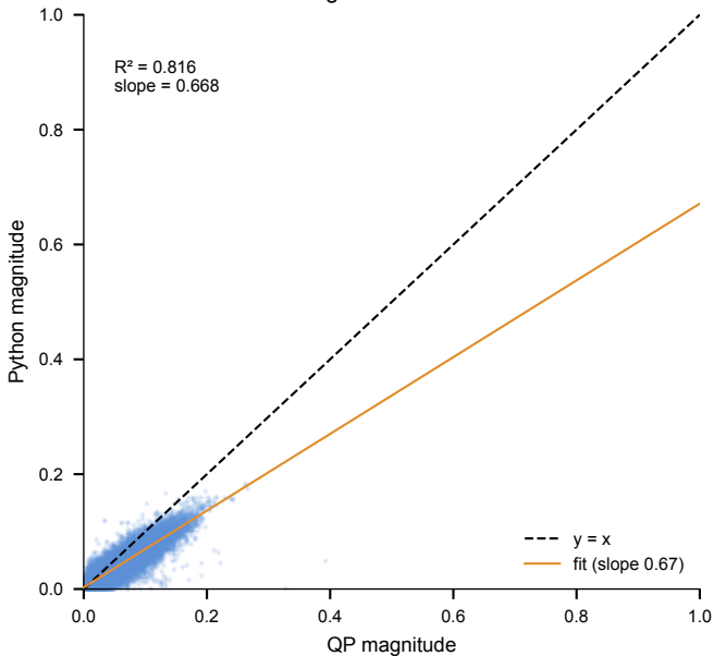
A Magnitude correlation
