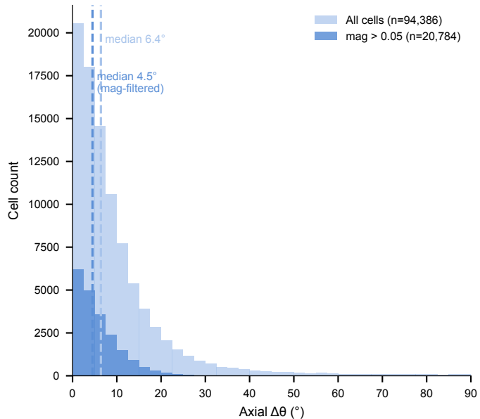
B Axis angle agreement (axial \Delta\theta )
