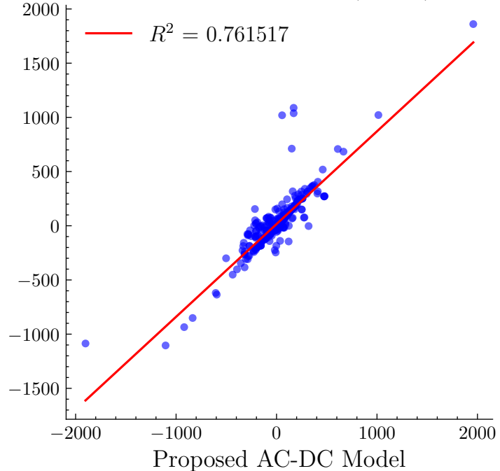
Reactive Power Flow (MVA r )
