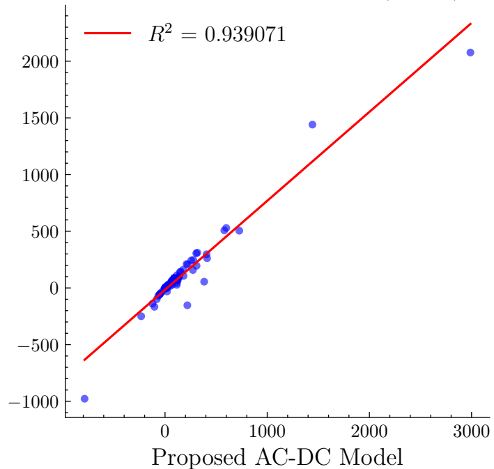
Reactive Power Generation (MVar)
