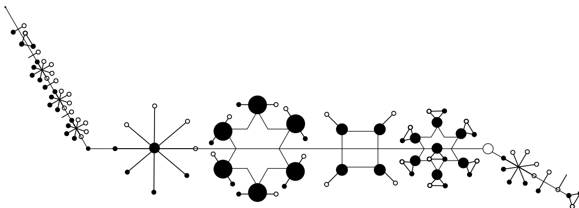
Figure 10.12: The x-LGES form rendering of the \Omega_{vuler} , the Euler Virus , now with HEAD , BODY and ROOT segments.
