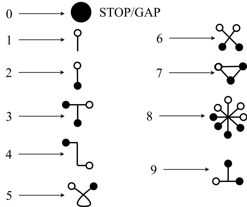
Figure 10.2: The OZIN Cipher[12], a mapping from Decimal Symbols (our base-Ω) to Symbols for Intermediate Genetic Code.
