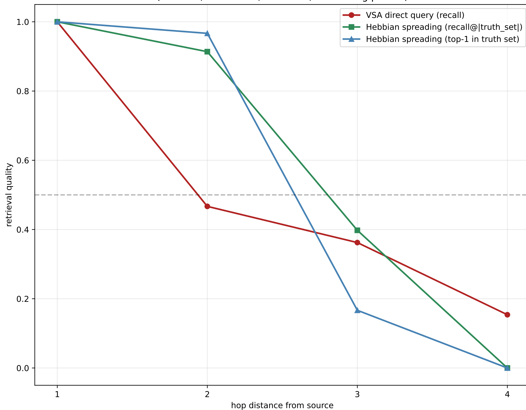
Connectivity vs structure: VSA query vs Hebbian spread (N=4096, 50 entities, 150 facts, 50 training passes)
