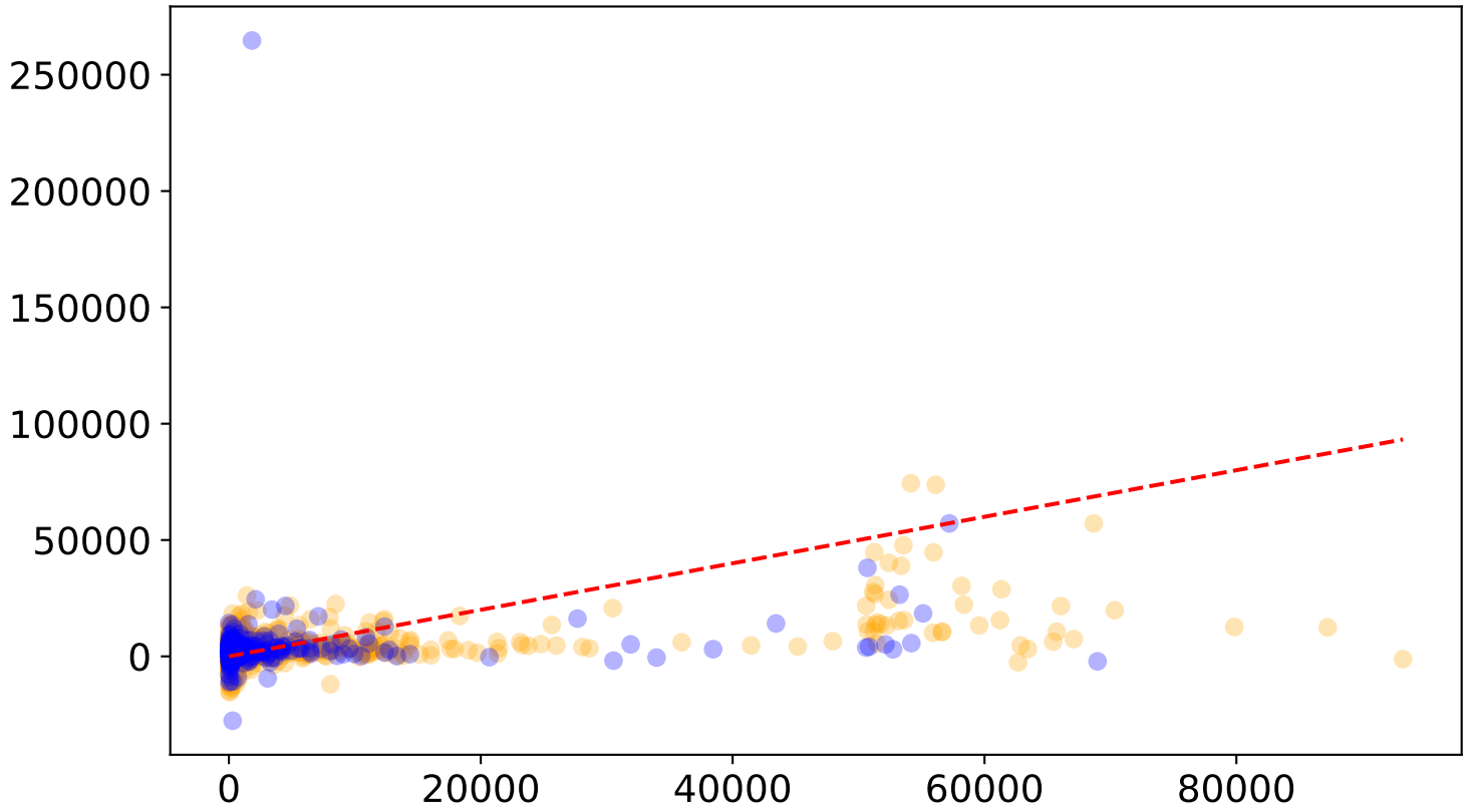
OLS Polynomial Features (No Lasso)
