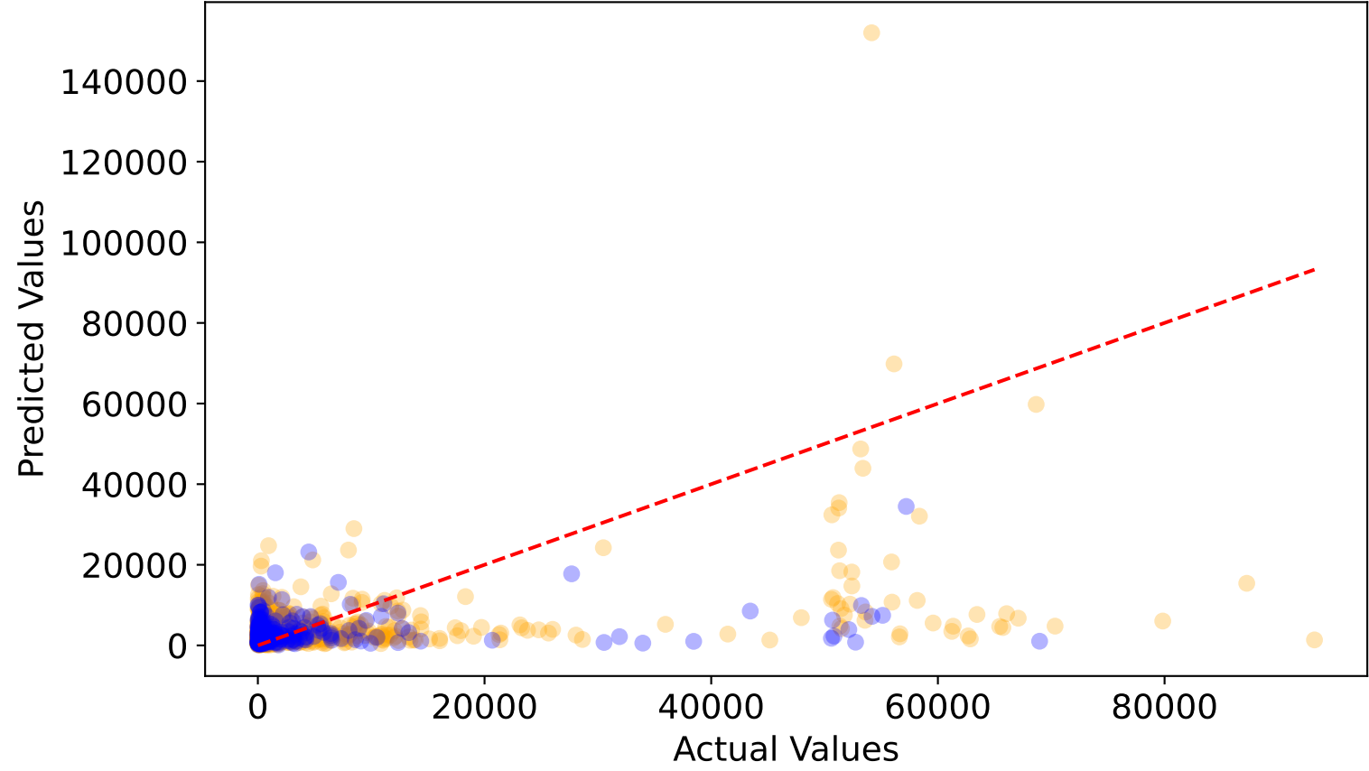
Poisson (No Ridge)
