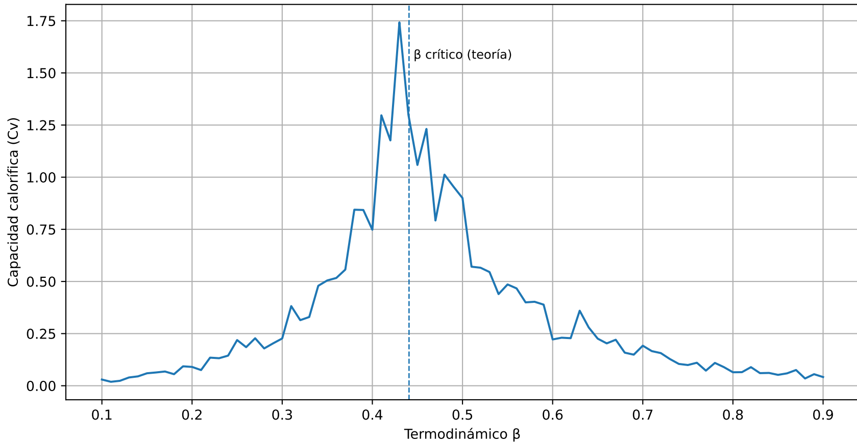
C_v(\beta) - Ising 2D Metropolis - N=20
