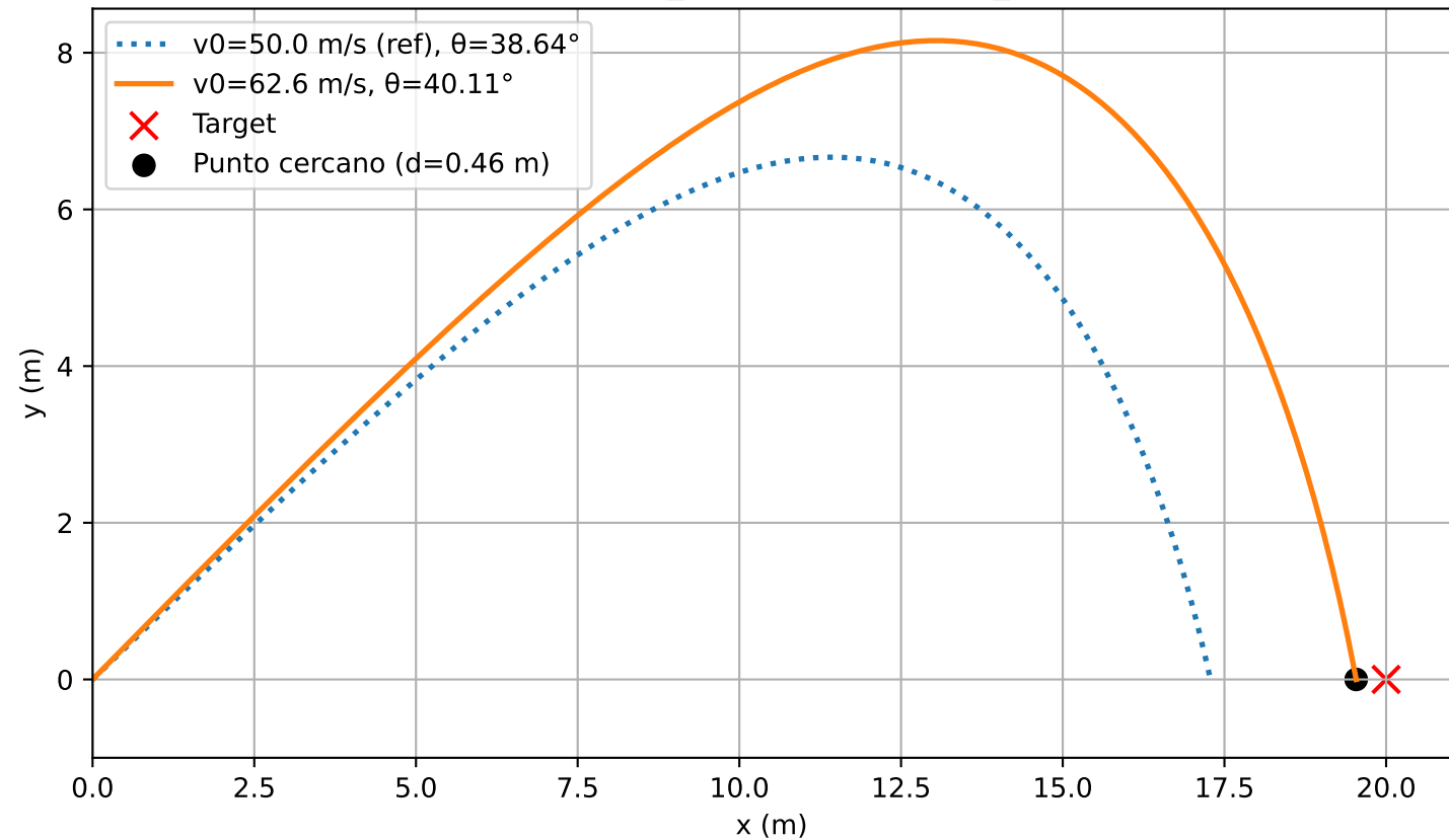
Target x=20.0 m — v0_ref=50.0 m/s vs v0_min=62.6 m/s
