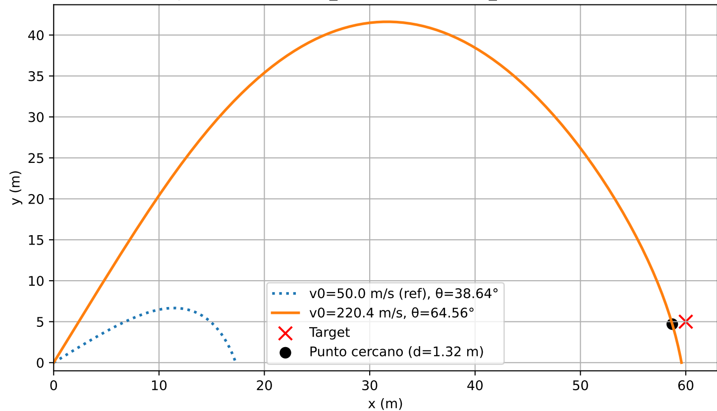
Target x=60.0 m — v0\_ref=50.0 m/s vs v0\_min=220.4 m/s
