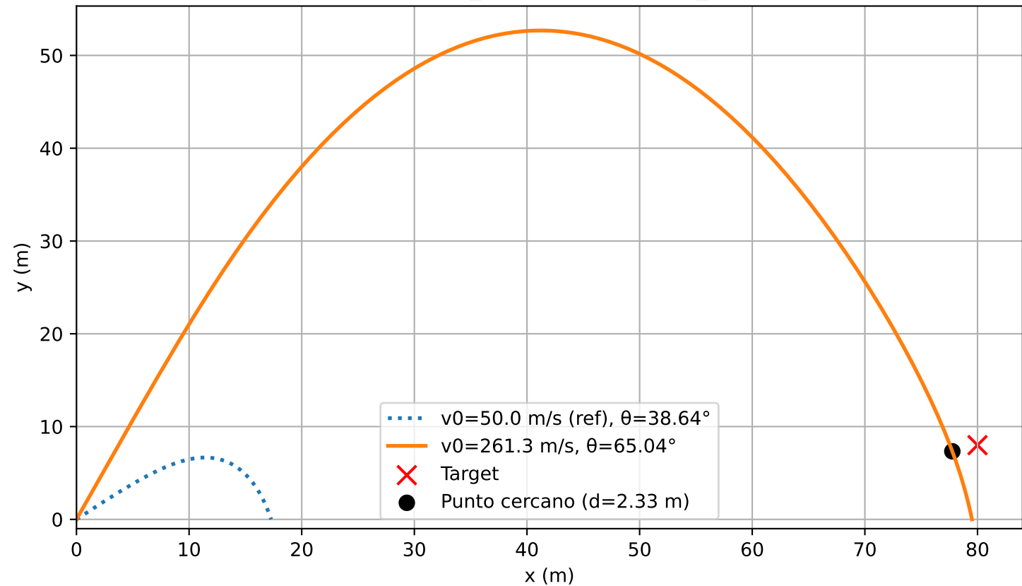
Target x=80.0 m — v0\_ref=50.0 m/s vs v0\_min=261.3 m/s
