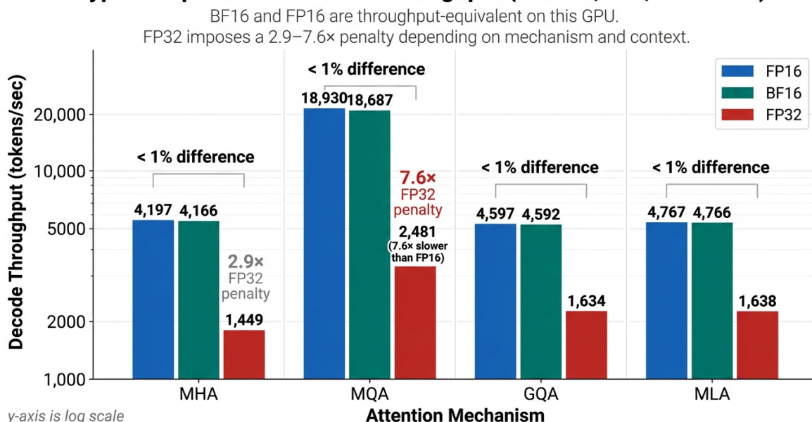
Figure 4: Decode throughput across dtypes (FP16, BF16, FP32) at context 8192, batch size 4. Each group of three bars corresponds to one attention mechanism. BF16 and FP16 bars are nearly indistinguishable; FP32 bars are 3–8× shorter. MQA’s FP32 bar shows the largest relative collapse, falling from 18,930 tok/s to 2,481 tok/s (7.6×).
