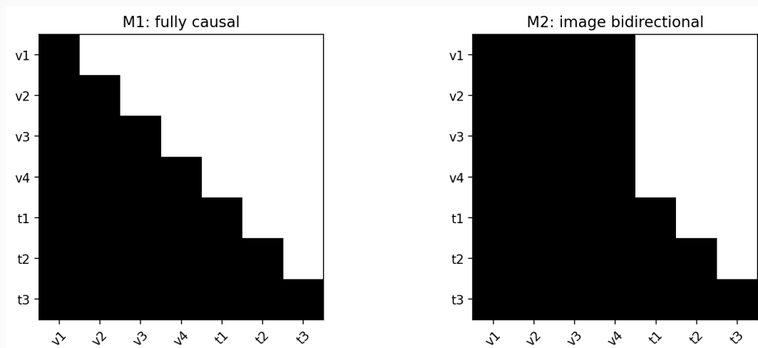
Figure 6: Attention masks for 4 visual + 3 text tokens. Left: fully causal (M1). Right: image bidirectional (M2). Shaded/white cells indicate allowed attention.
