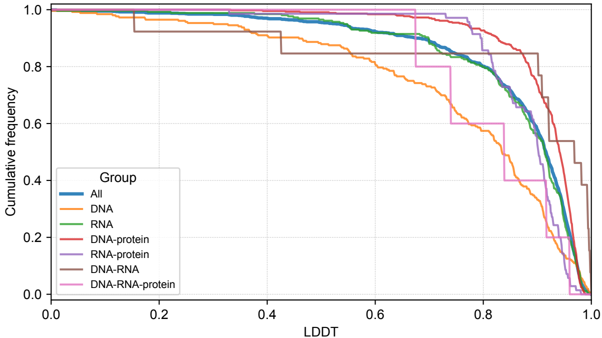
Cumulative frequency — LDDT
